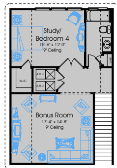
Optional Bonus Room and Bedroom 4 +668 Sq. Ft.
