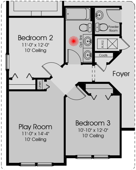
Optional Play Room (Also shown: Opt. 2nd sink at hall bath AND Opt. Powder Room)
