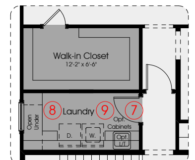
Optional Cabinets at Standard Laundry Room
