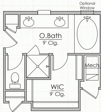
Optional Deluxe Owner's Bath +5 Htd. Sq.Ft.
