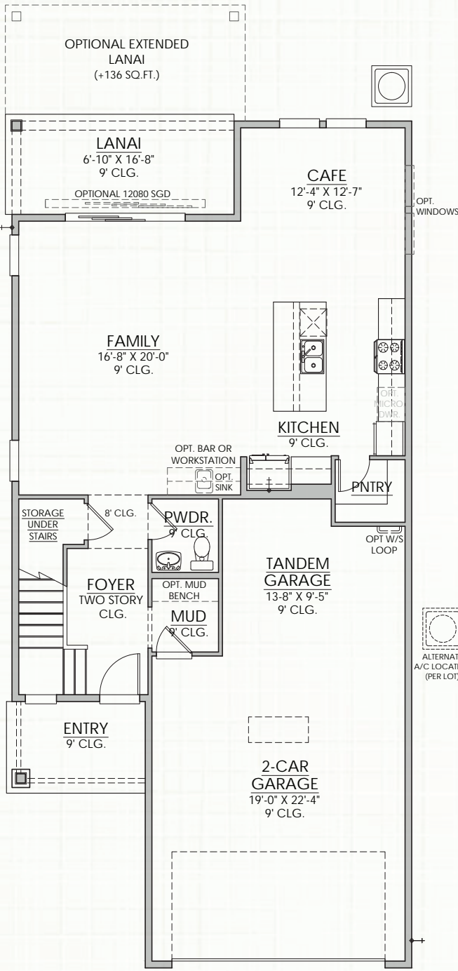
1ST FLOOR PLAN (Elevation E)
