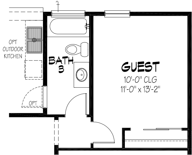
OPT GUEST & BATH 3
